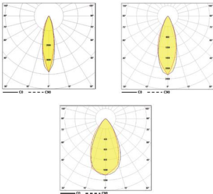
Beam Angle for Pluto-P & Pluto-ST
