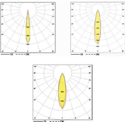
Beam Angle for Pluto-P & Pluto-ST
