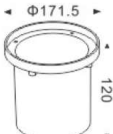
Mounting Sleeve
